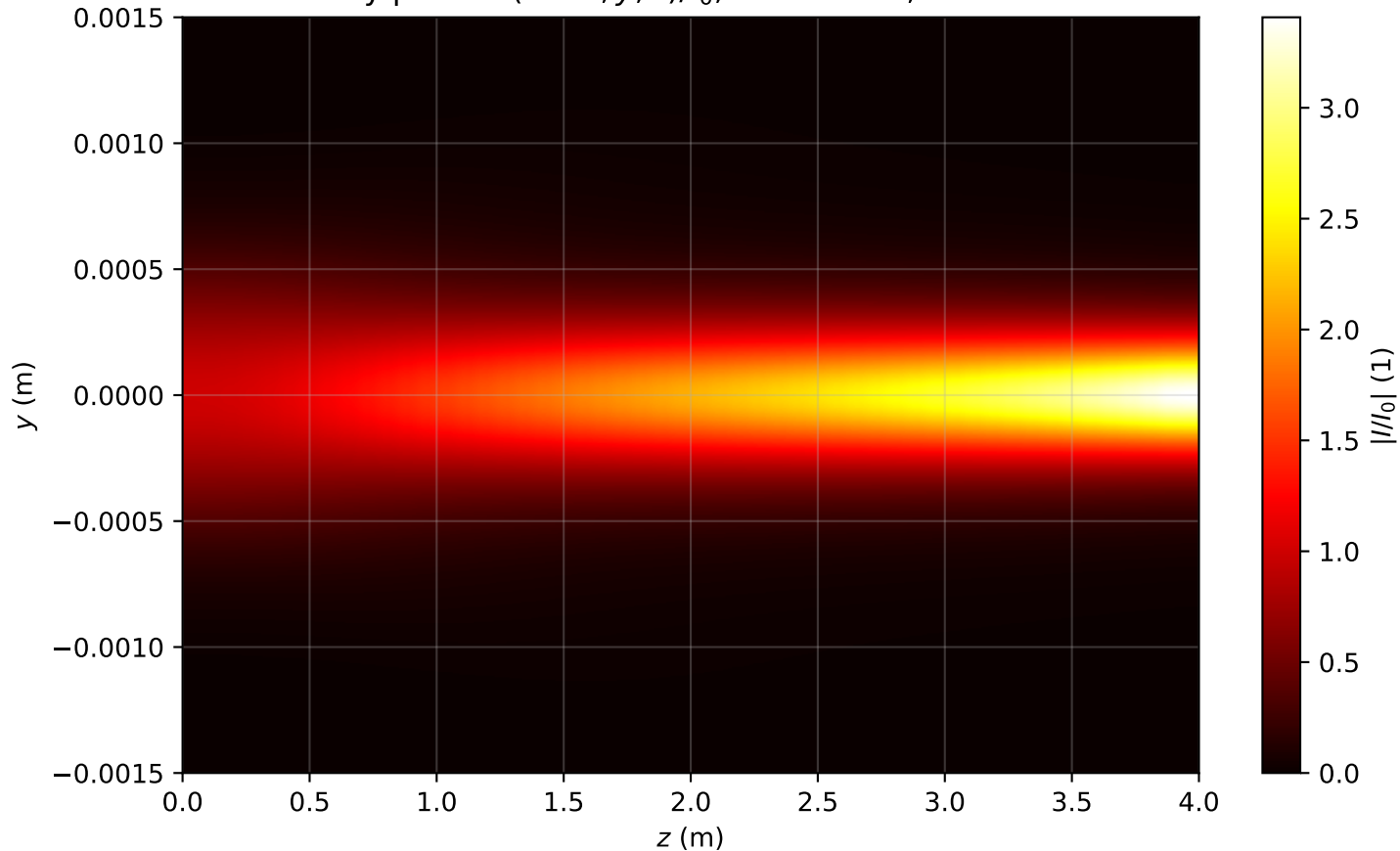
Intensity profile I(x=0, y, z)/I_0 , P_{in}=1.0P_{cr} , artificial time
